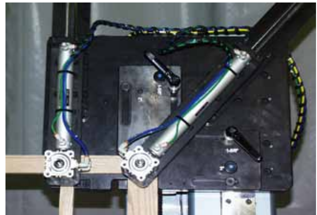
Adjustable clamp pads accommodate 1-1/2" to 4-1/2" stile and rail sizes at 1/4th" increments
